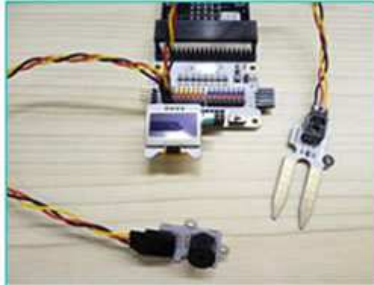
Soil moisture detection
